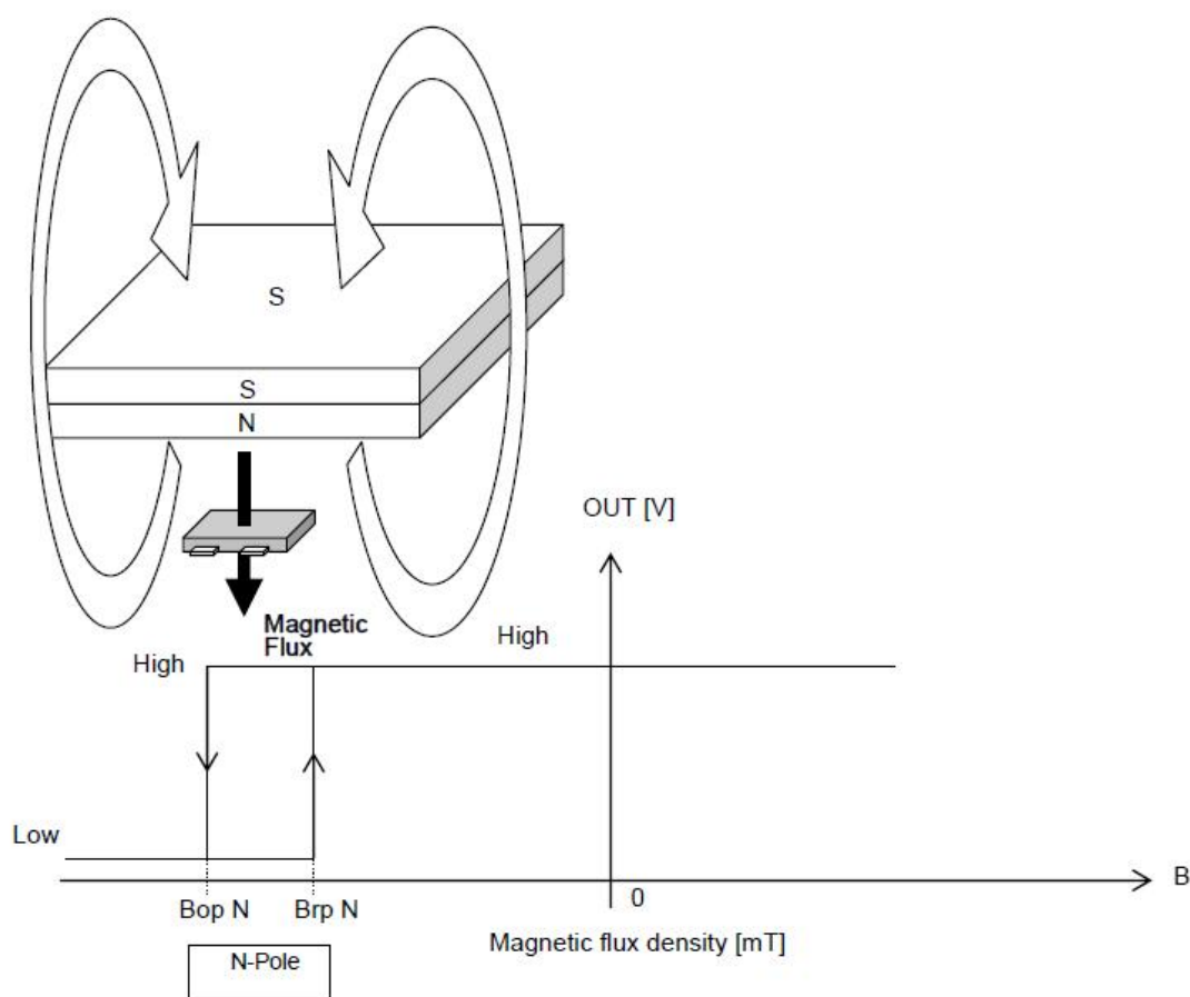
Fig 4, Magnetic Operation Characteristic of AS1911
