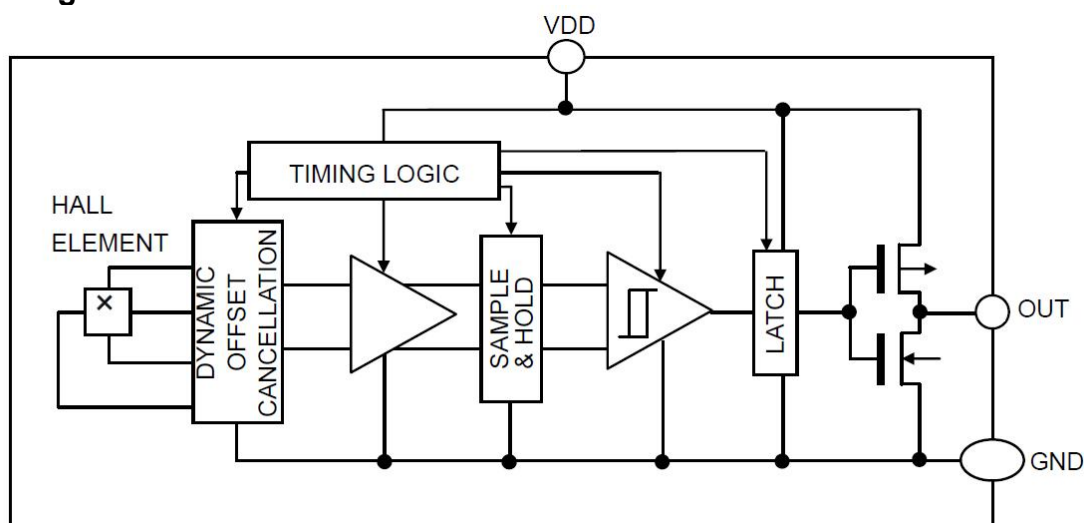
Figure 3, Block Diagram of AS1911
